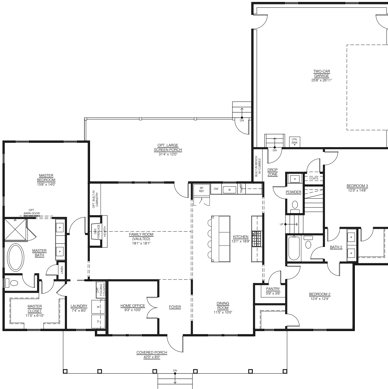
THE WATSON GROUND FLOOR PLAN - 2,282 SF
